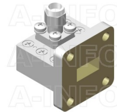
51WCA3.5M_Cu Right Angle Rectangular Waveguide to Coaxial Adapter 15-22GHz WR51 to 3.5mm Male
